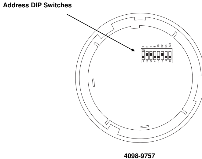
Figure 3-11. Location of DIP Switches on QuickConnect Sensor
