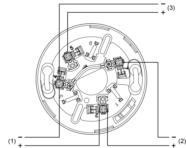
Figure 1: Wiring the SIGA-SB
