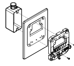
One-gang Electrical Box
