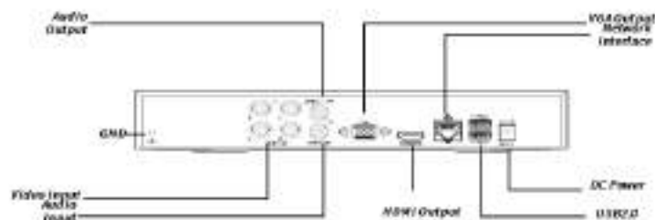
[XVR301-08G3]
